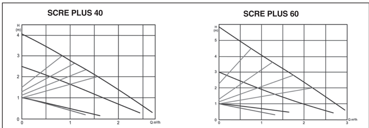
pumps performance curves
